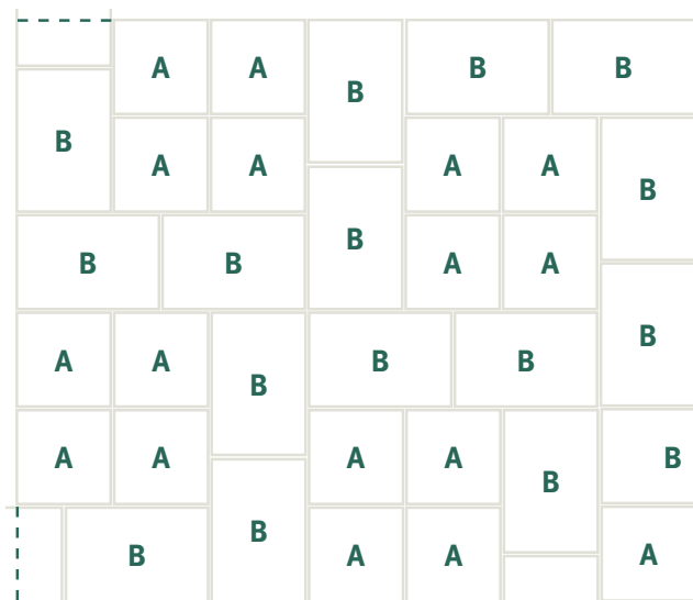
Blockverband
